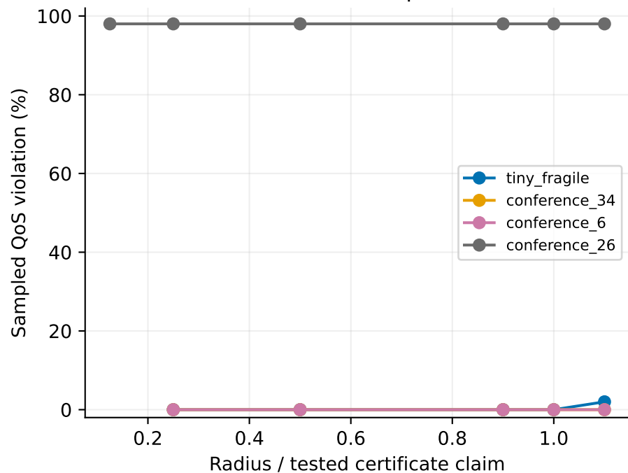
Monte Carlo counterexamples (n=50/seed)
