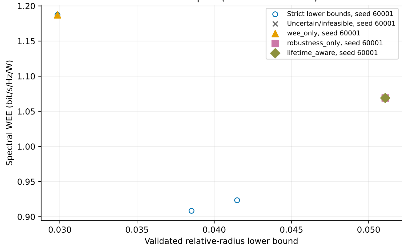
Full candidate pool (direct intercell ON)
