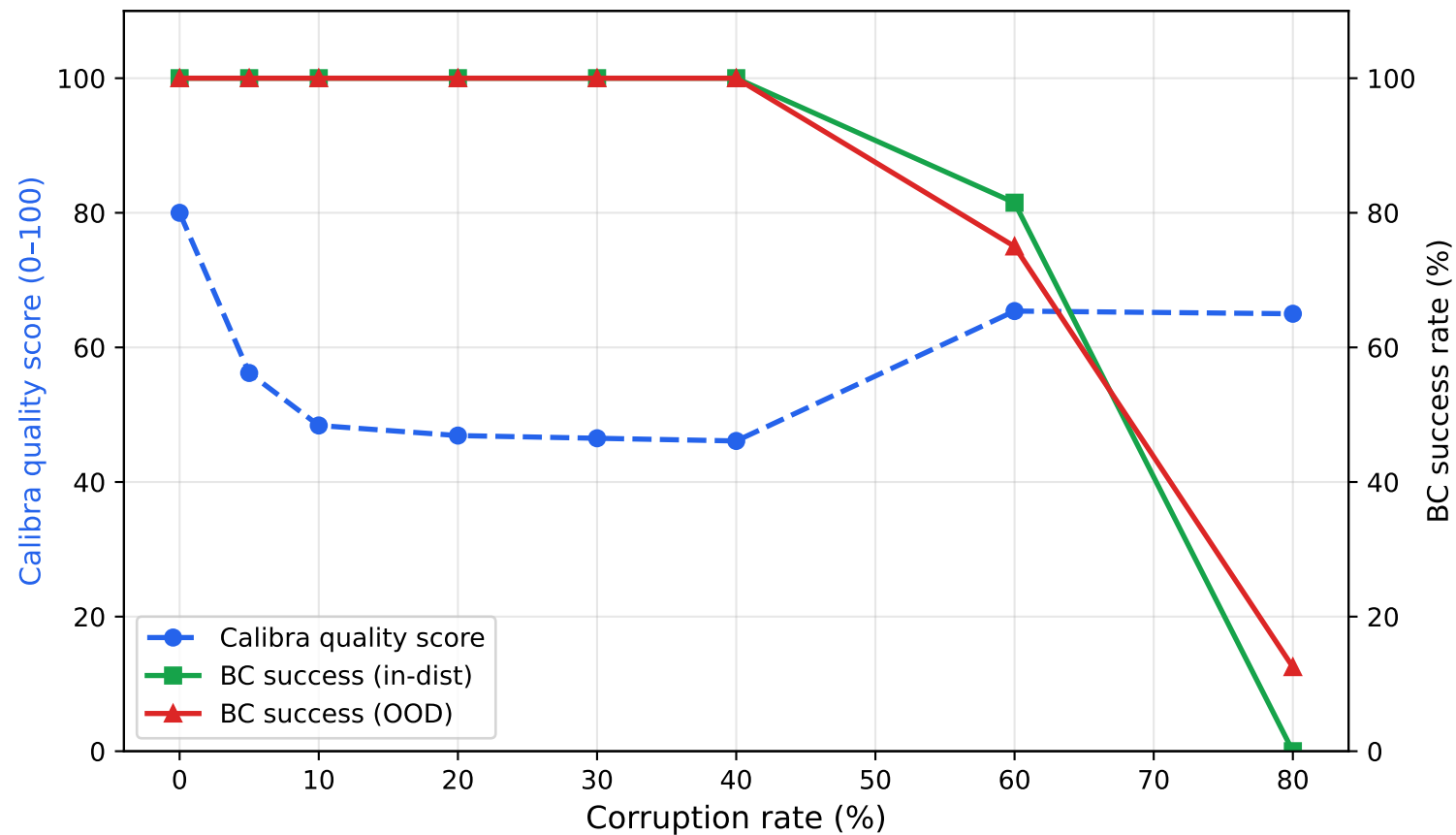
IL Ceiling Experiment — Calibra quality score tracks BC success ceiling
