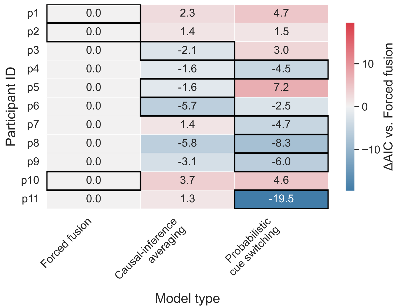
B Model comparison with free sensory-noise parameters
