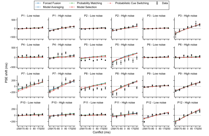
Figure 12: This is exactly the same as Figure ??, except that here the models are fitted using the sensory-noise parameters ( \sigma_{a,l} , \sigma_{a,h} , \sigma_v ) that were estimated based on the psychometric fits to the unimodal data.
