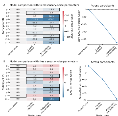
Figure 10: (A) Model comparison assuming sensory-noise parameters fixed to values estimated from the unimodal tasks. (B) Model comparison when sensory-noise parameters were fit to the bimodal data. Left panels show participant-level \Delta AIC values for each model, computed relative to the forced-fusion model (the baseline column, which is therefore identically zero); negative values (blue) indicate a better fit than forced fusion. Rows correspond to participants and columns correspond to models, and the best-fitting model (lowest AIC) for each participant is outlined. When sensory-noise parameters were fixed (A), the probabilistic cue-switching model provided the best fit for 8 of 11 participants. When the sensory-noise parameters were fit directly to the bimodal data (B), the cue-switching model provided the best fit for 6 of 11 participants.
