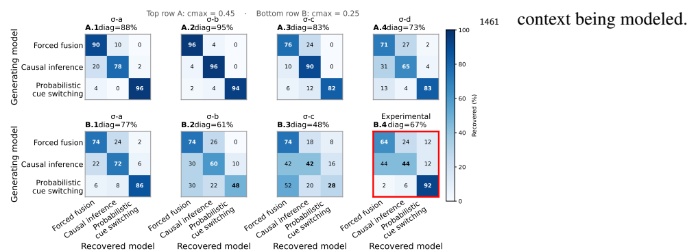
Figure 19: Model recovery across sensory-noise and conflict regimes.
