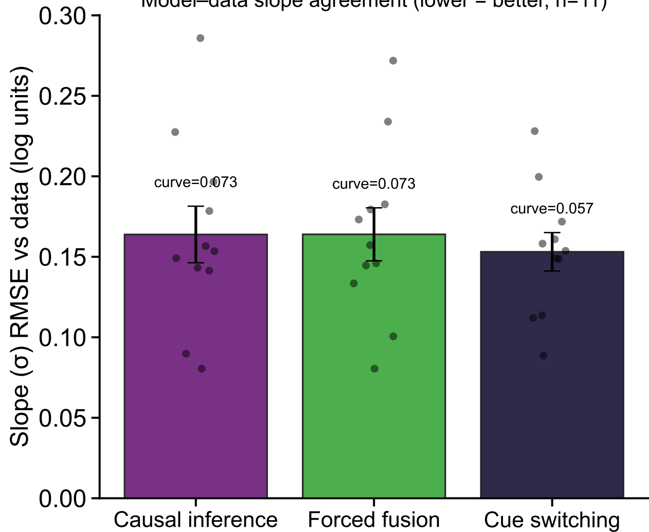
Model-data slope agreement (lower = better, n=11)
