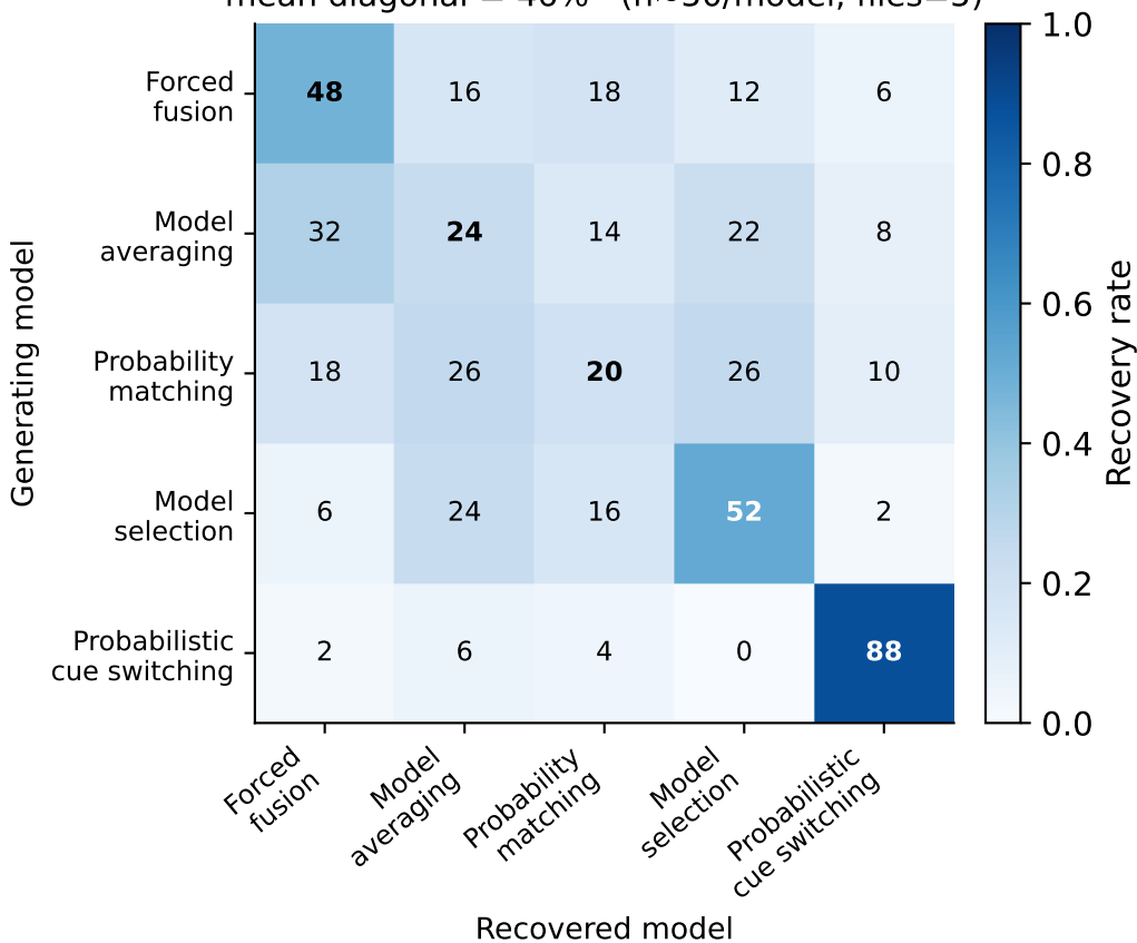
Empirical recovery — 5 models (AIC) mean diagonal = 46% (n≈50/model, files=5)
