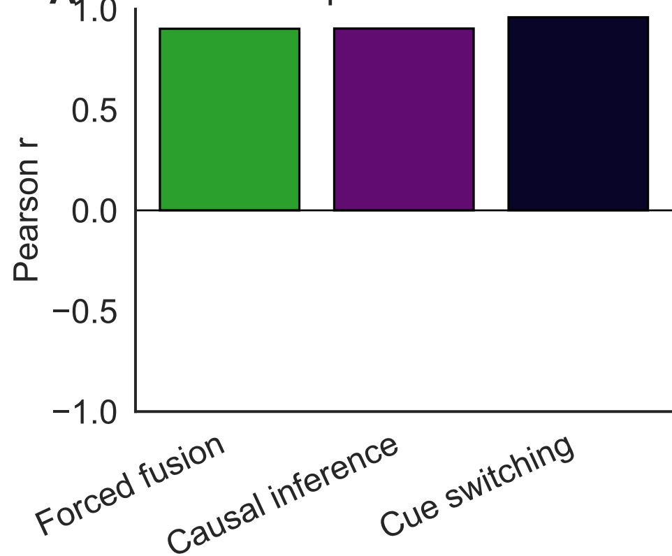
A Simulated-response noise correlation
