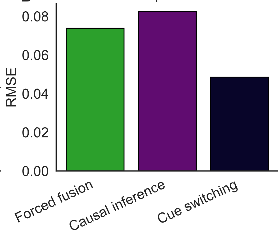
B Simulated-response noise error
