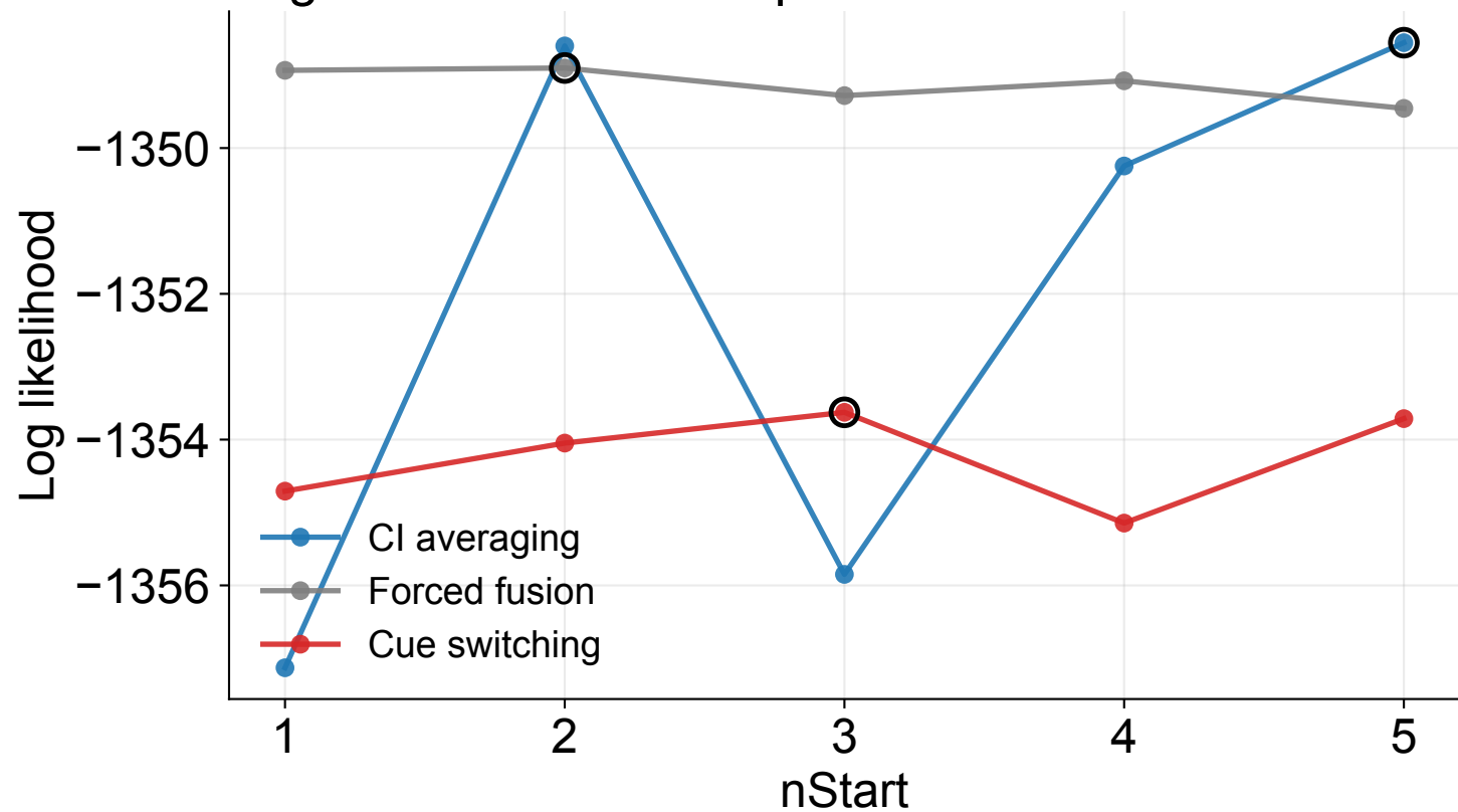
Log likelihood across optimizer starts
