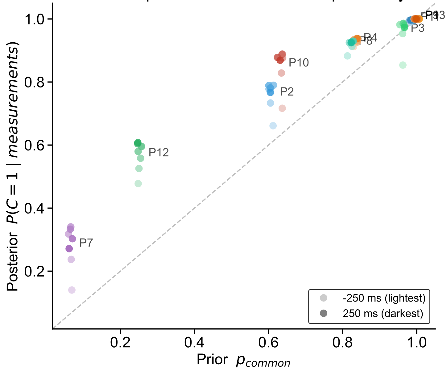
Prior vs. posterior common-cause probability
