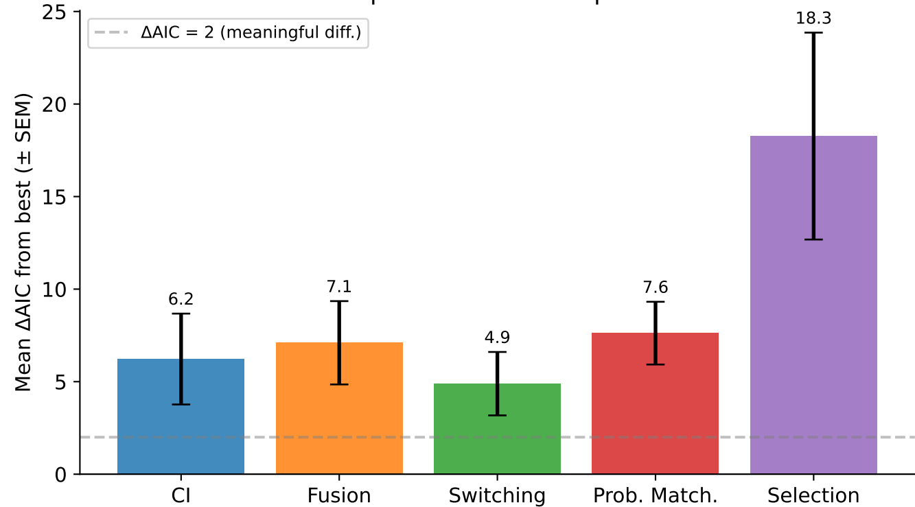
Group-level model comparison
