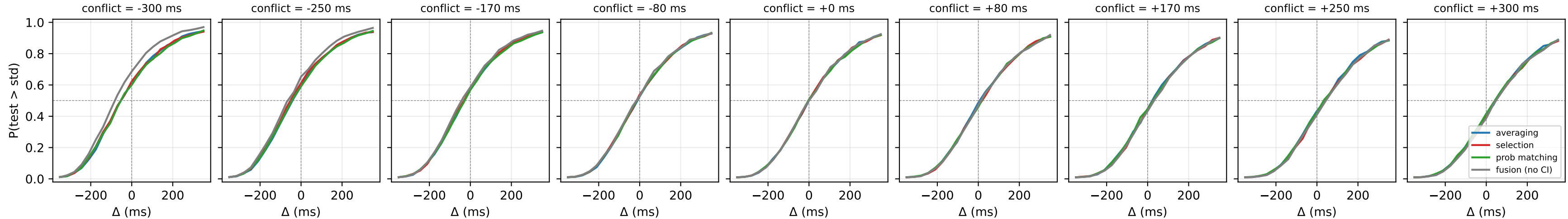
Predicted PFs per conflict — low_aud_noise
