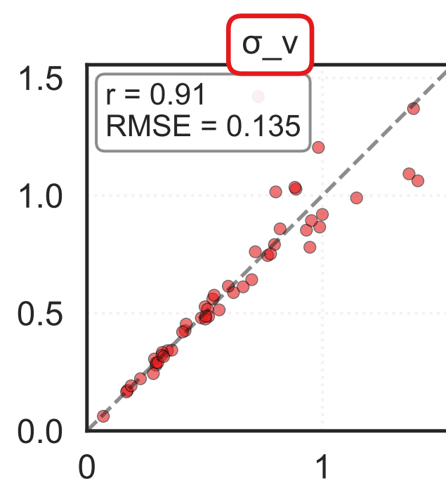
Parameter Recovery – Free/Wide-Range Params (X: Generating, Y: Recovered)
