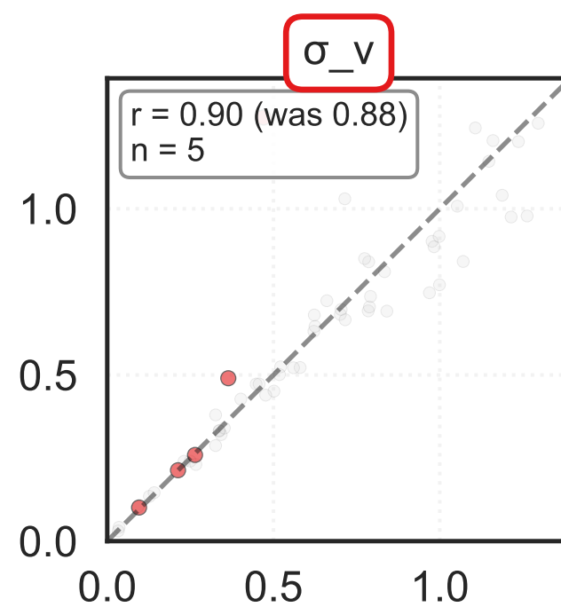
Parameter Recovery – Filtered with \sigma_a, \sigma_v \leq 0.5 (grey = excluded, colour = kept)
