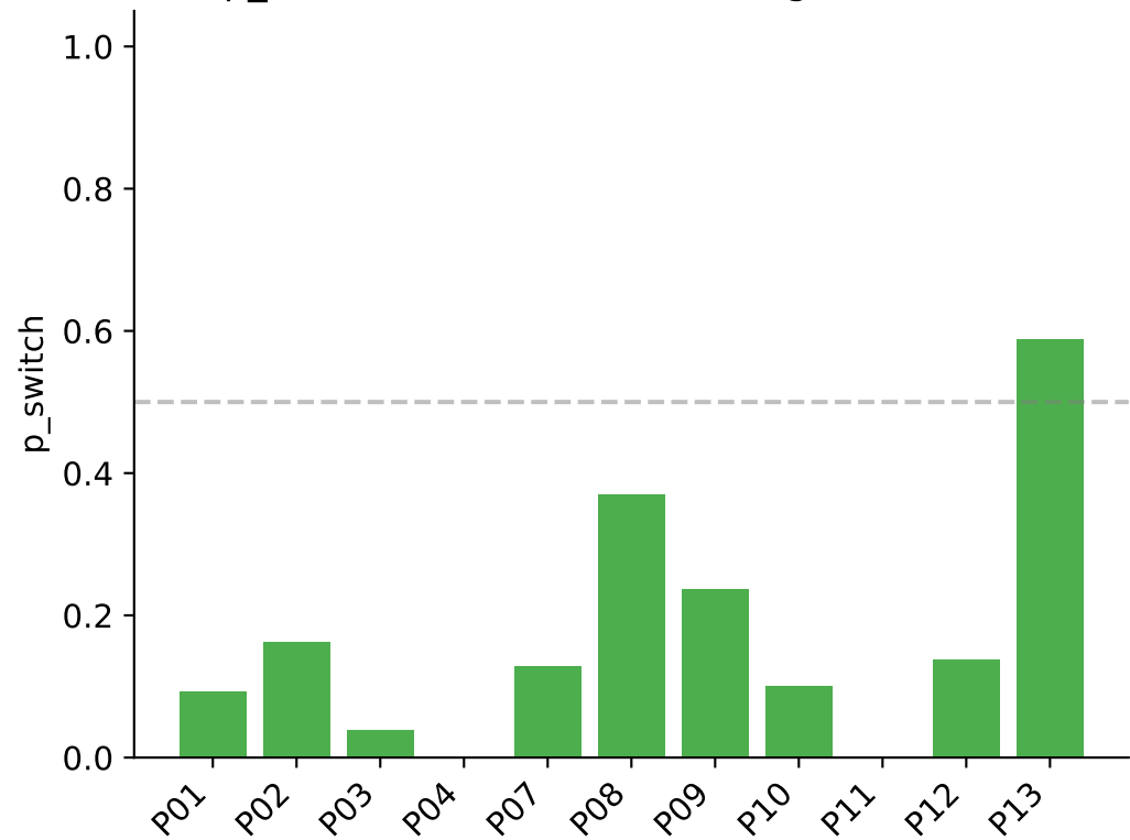
p_switch estimates (SwitchingFree model)
