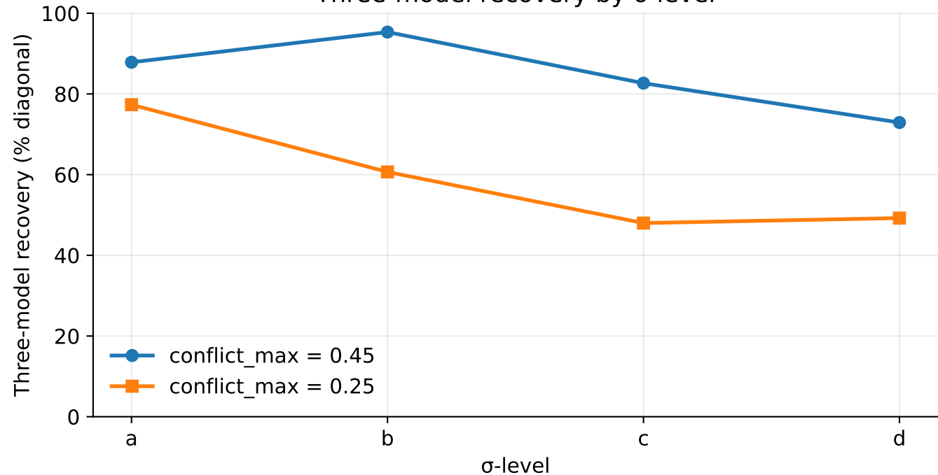
Three-model recovery by \sigma level
