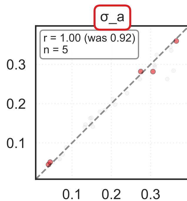
Parameter Recovery – Filtered with \sigma_a, \sigma_v \leq 0.5 (grey = excluded, colour = kept)
