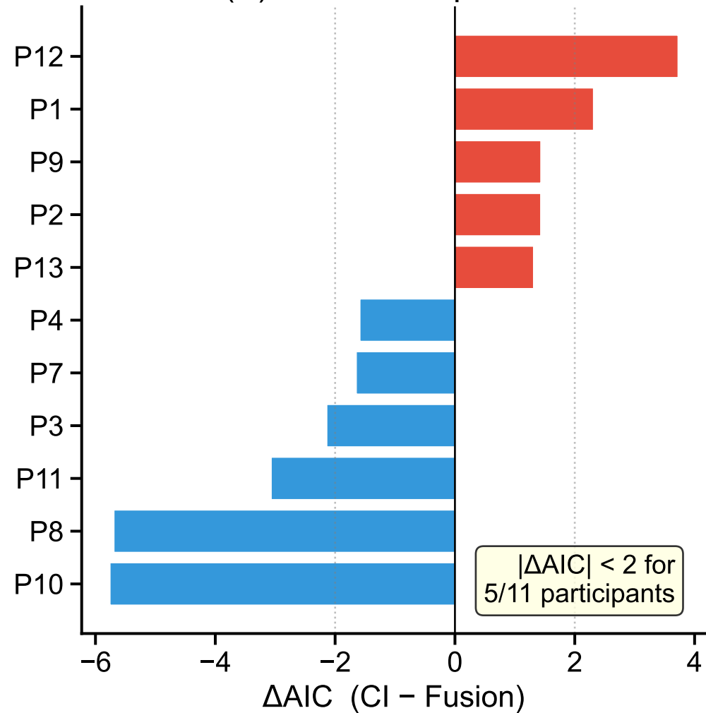
(A) Model comparison
