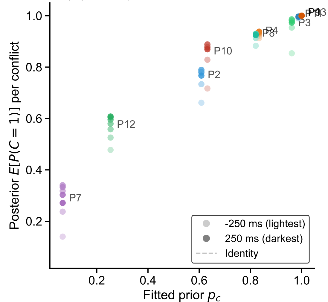
(C) Prior p_c vs. posterior per conflict
