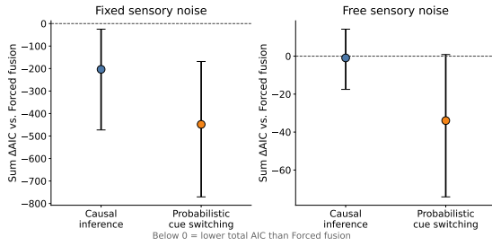
Figure 10: Group-level model comparison: summed \Delta\text{AIC} . Sum of the per-participant \Delta\text{AIC} relative to the forced-fusion model (the baseline, fixed at 0 and not shown) under fixed (left) and free (right) sensory noise. Each colored point is the total across the 11 participants for one model, with 95% confidence intervals from 10,000 participant bootstrap resamples. Values below the dashed zero line indicate a lower total AIC, i.e. a better fit, than forced fusion. Under fixed sensory noise, the probabilistic cue-switching and causal-inference models fit clearly better than forced fusion (intervals below zero); under free sensory noise the totals are much smaller and the confidence intervals overlap zero.
