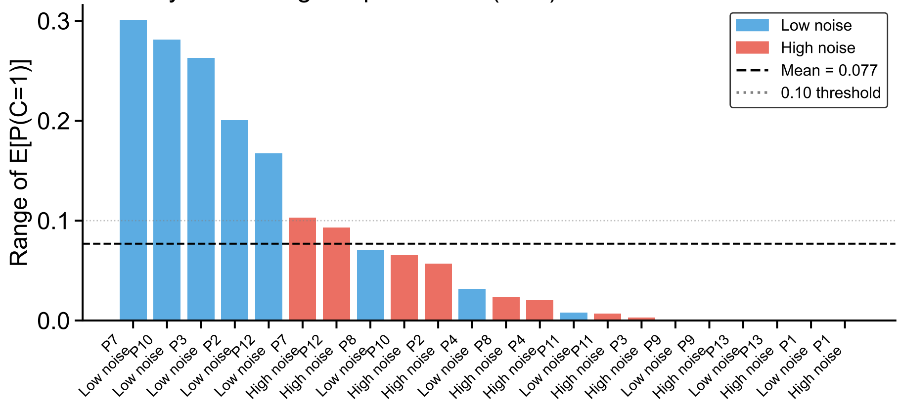
Dynamic range of posterior P(C=1) across 7 conflict levels
