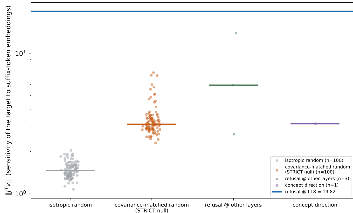
FIGURE B — local token reachability, test n=37 refusal is the MOST reachable direction, above every control family
