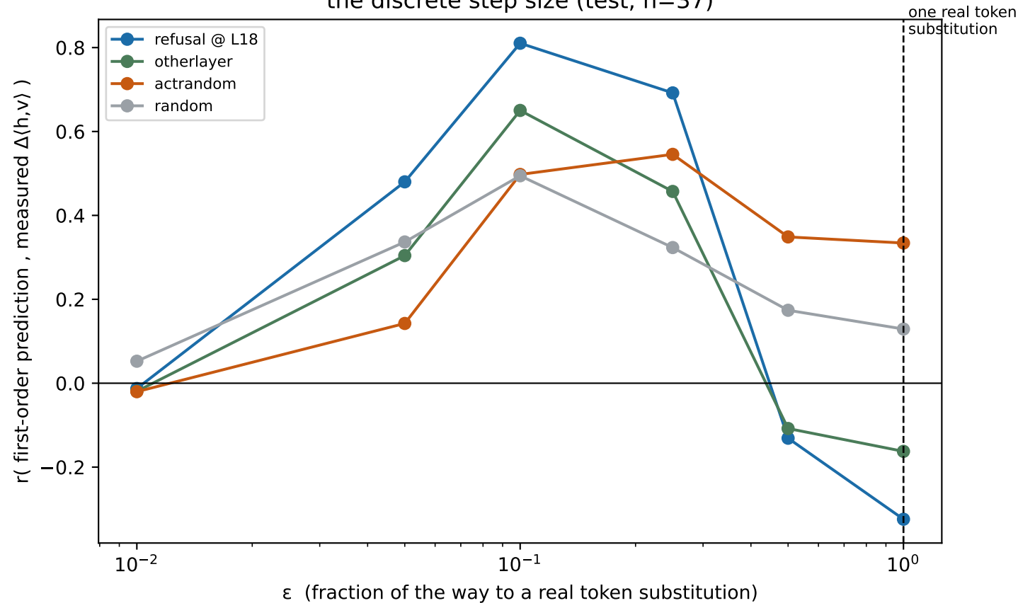
FIGURE B2 — GATE B: the linear surrogate GCG relies on is valid only far below the discrete step size (test, n=37 )
