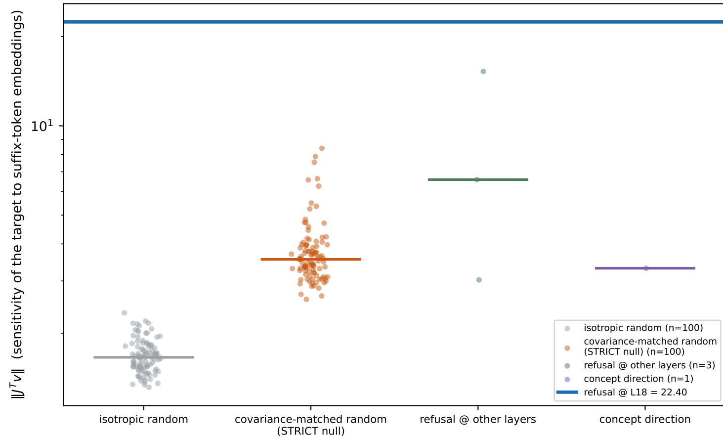
FIGURE B — local token reachability, train n=40 refusal is the MOST reachable direction, above every control family
