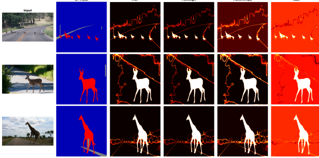
Figure 1. Qualitative comparison of anomaly score maps on Road-Anomaly21. Each row shows an input image alongside score maps produced by MSP, MaxLogit, MaxEntropy, and RbA for EoMT-Cityscapes.
