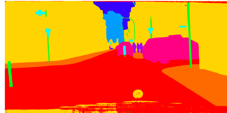
EoMT-Cityscapes
