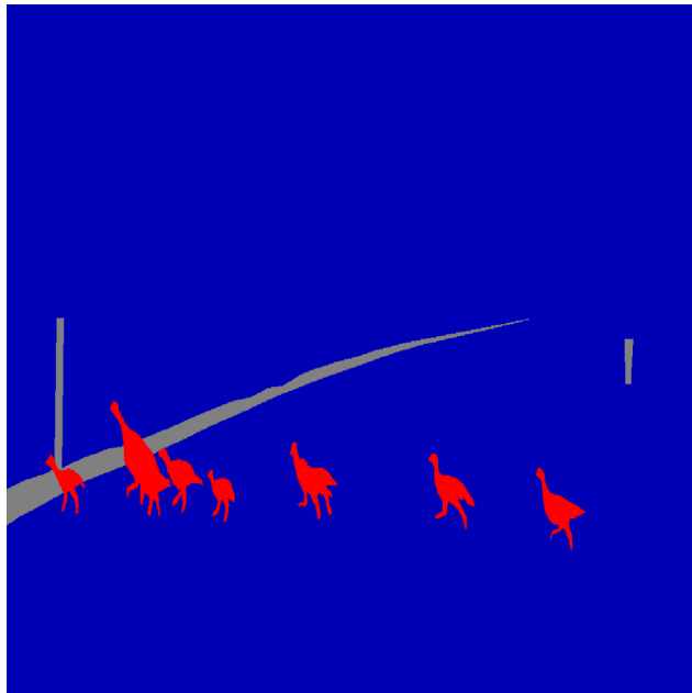
GT Mask
