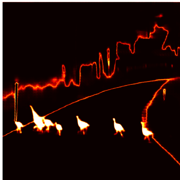
MSP
