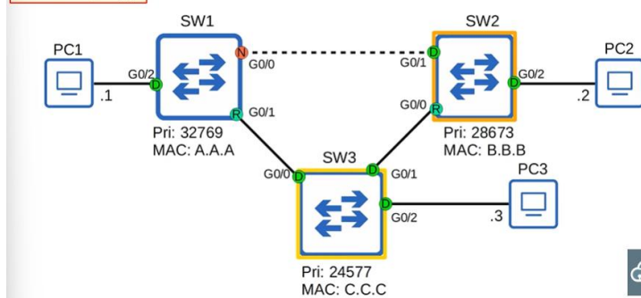
VLAN 1 Topology
