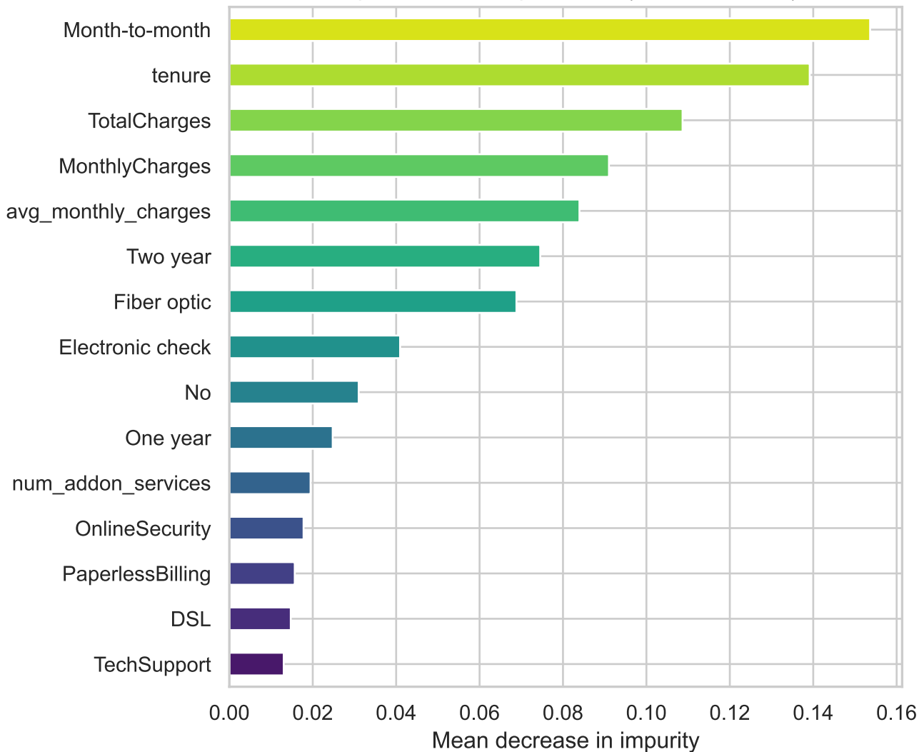
Top 15 Feature Importances (Random Forest)
