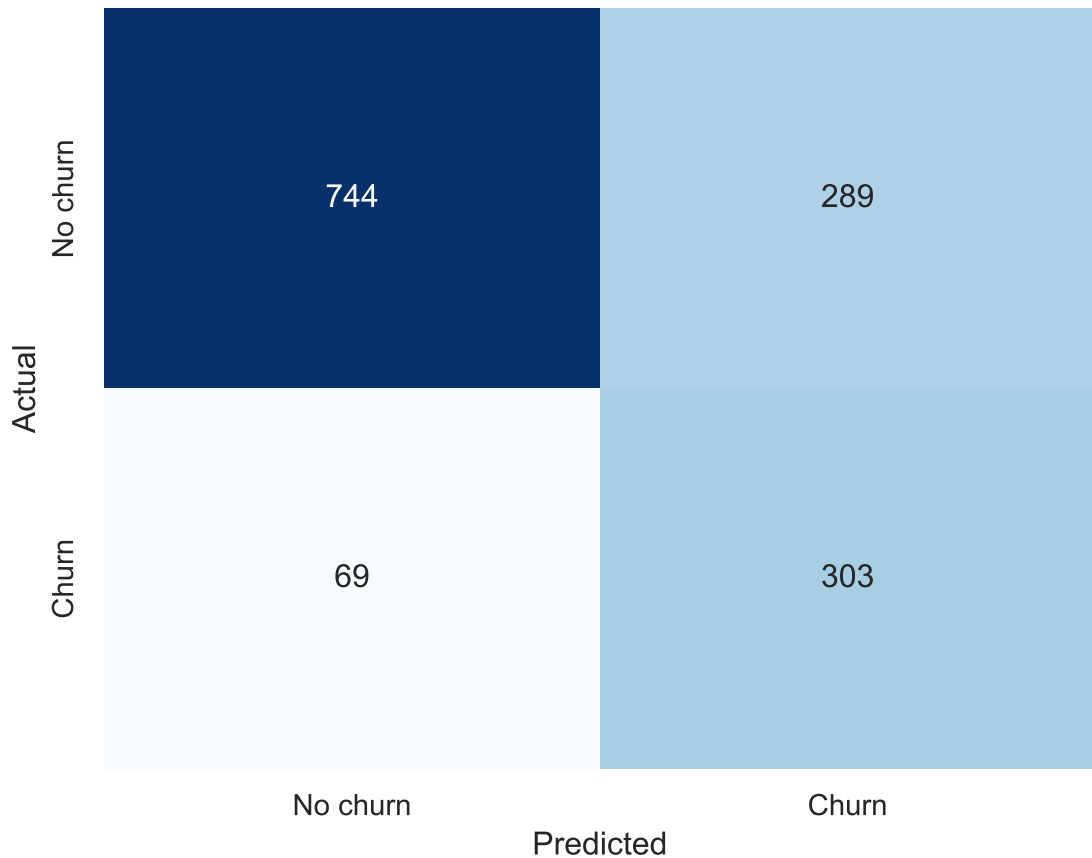
Confusion Matrix (threshold = 0.41)
