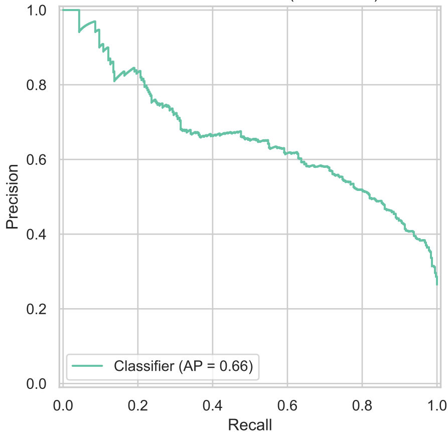
Precision-Recall Curve (AP = 0.658)
