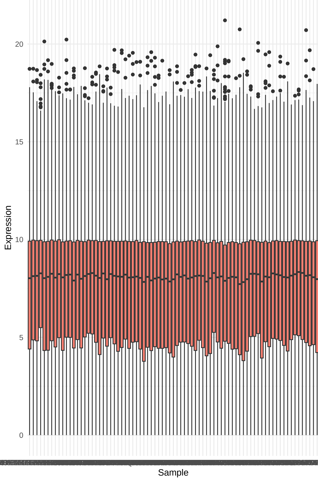
Boxplot \log_2(\text{TPM} + 1) filtered
