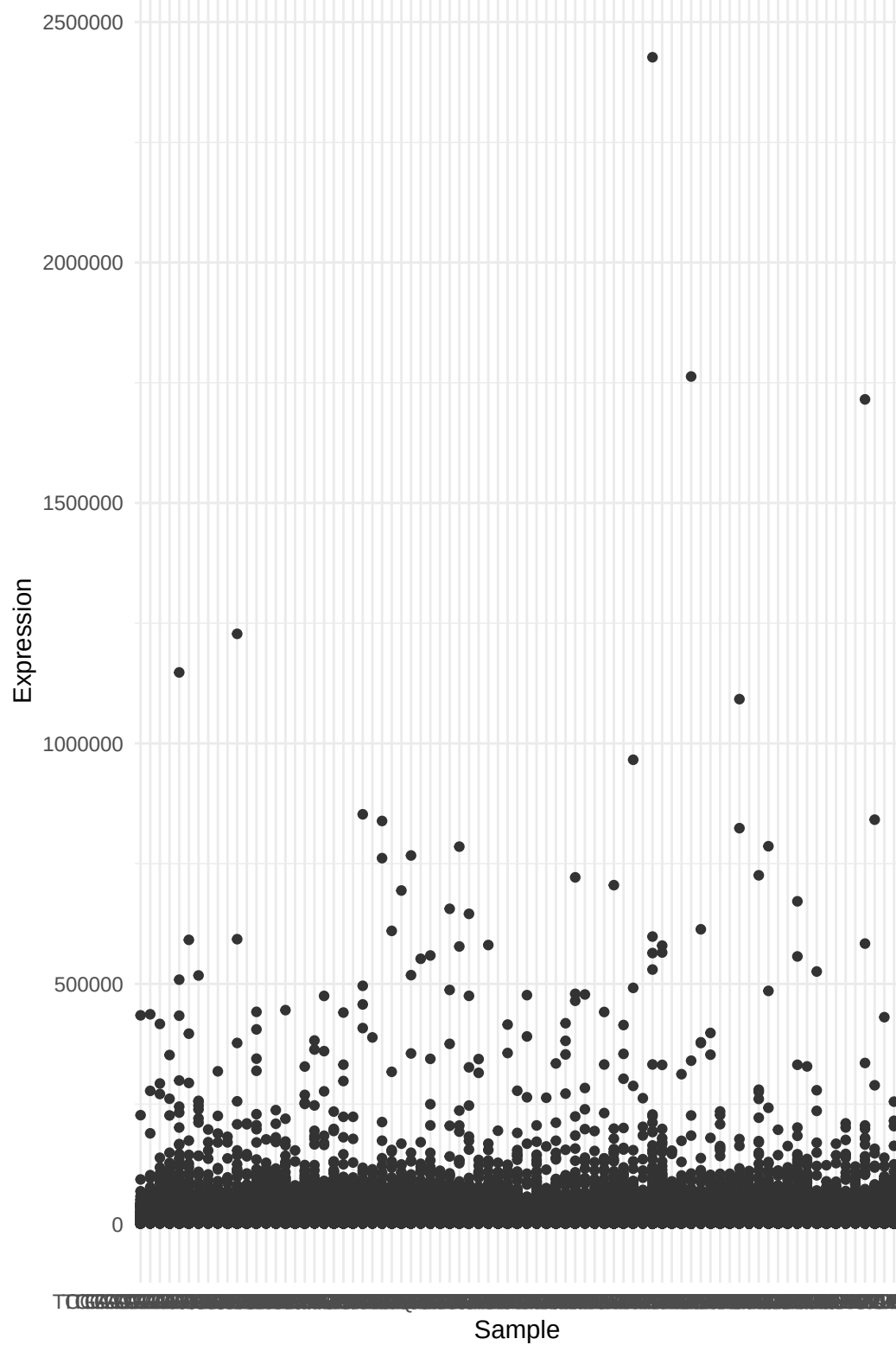
Boxplot TPM
