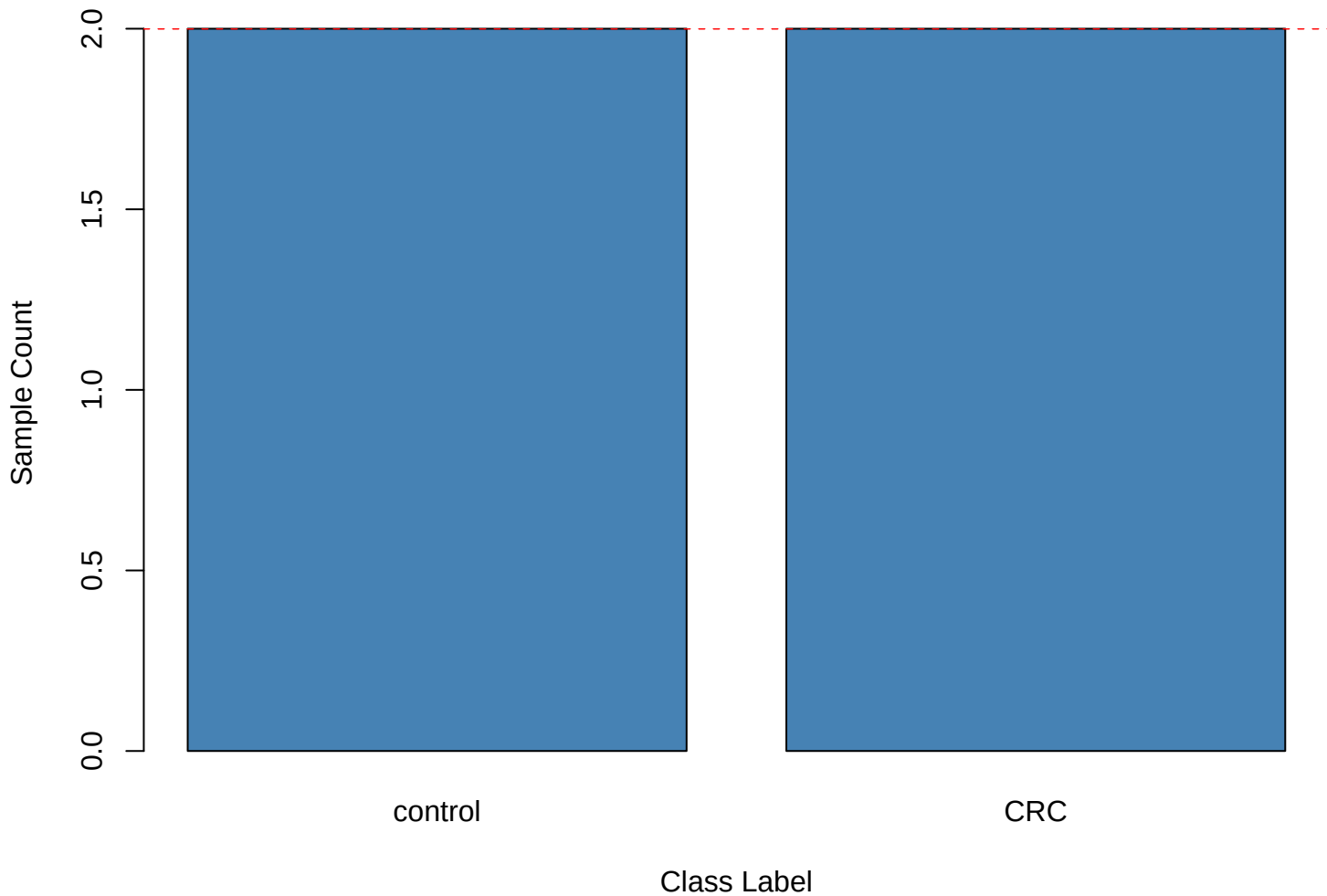
Class Distribution
