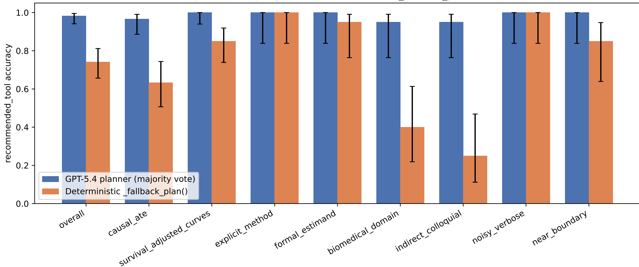
GPT-5.4 planner (majority vote) vs. deterministic _fallback_plan() baseline
