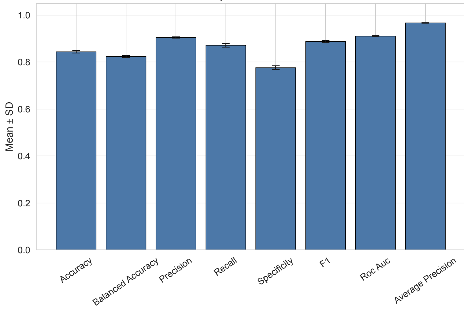
ET: Bootstrap Trial Mean Metrics \pm SD
