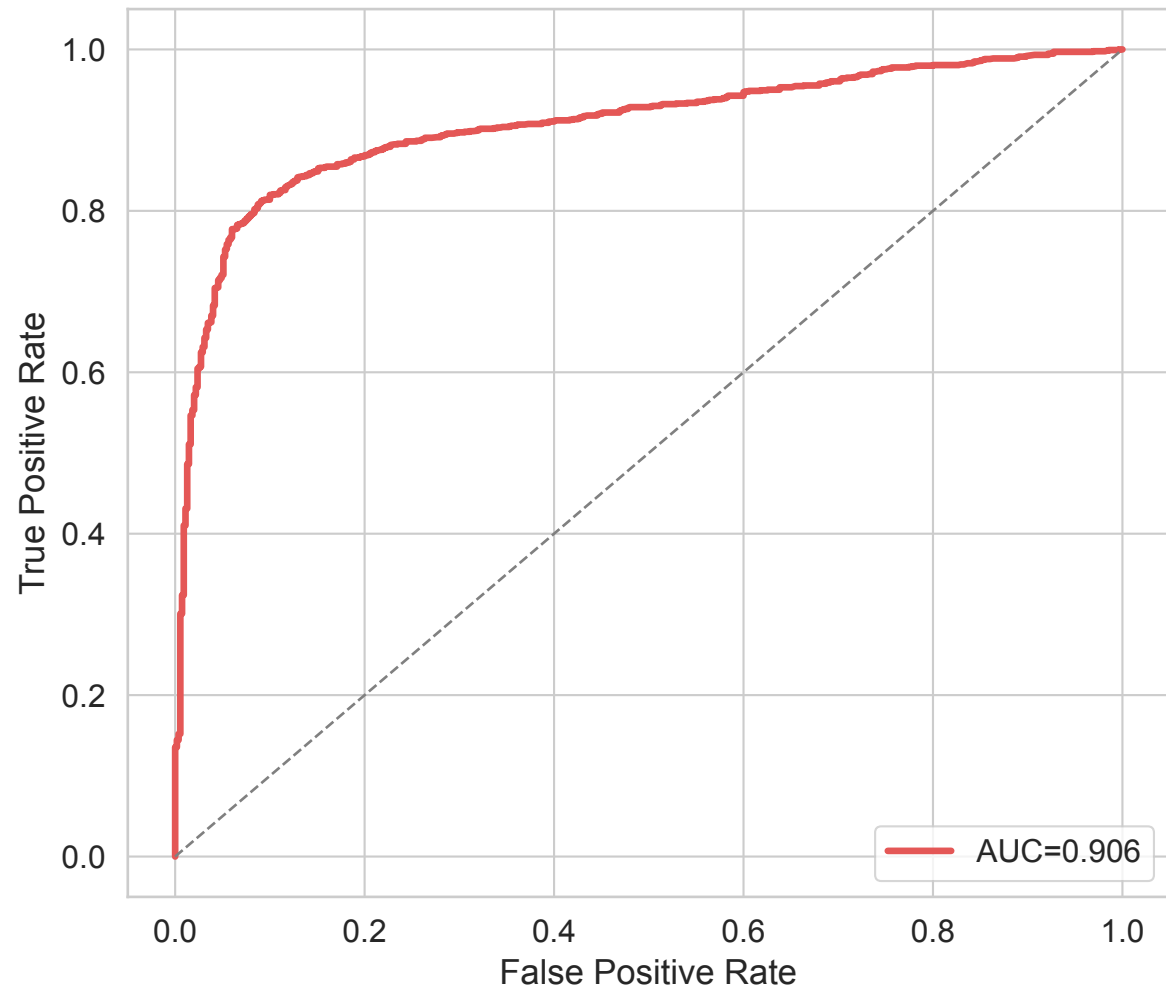
LGBM: ROC Curve
