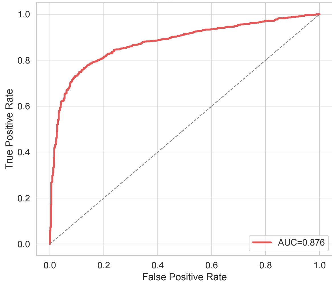
LogReg: ROC Curve
