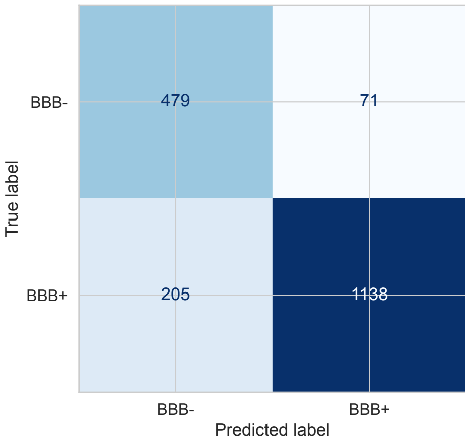
XGB: Confusion Matrix
