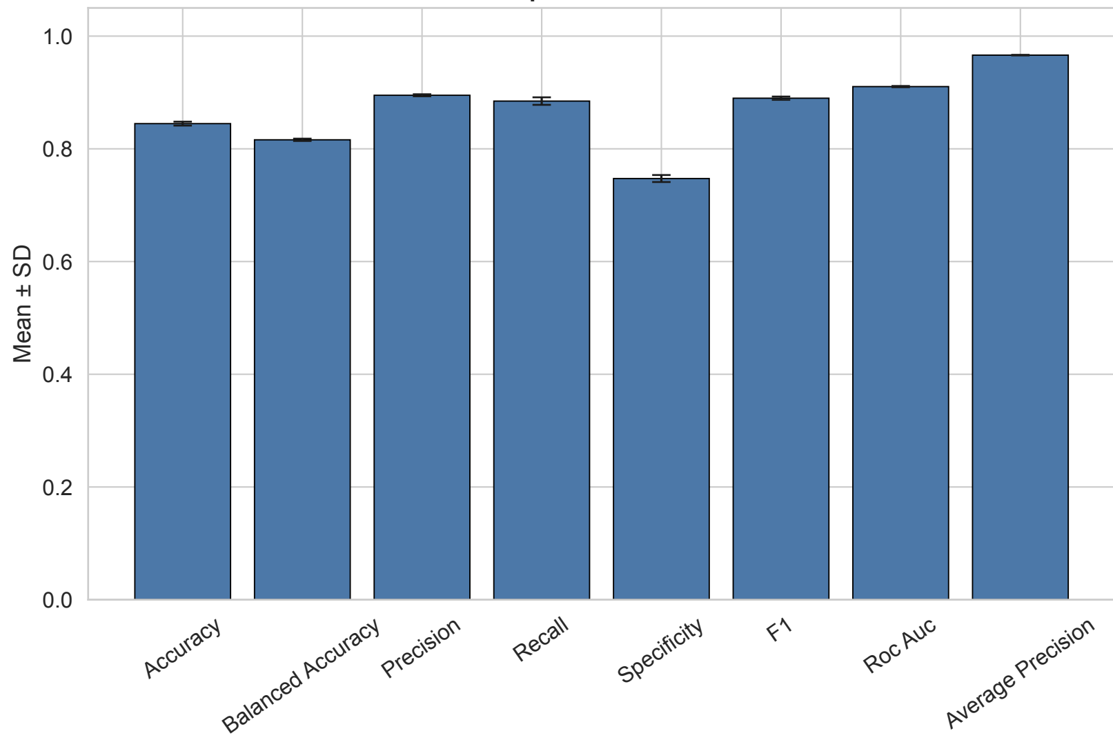
RF: Bootstrap Trial Mean Metrics \pm SD
