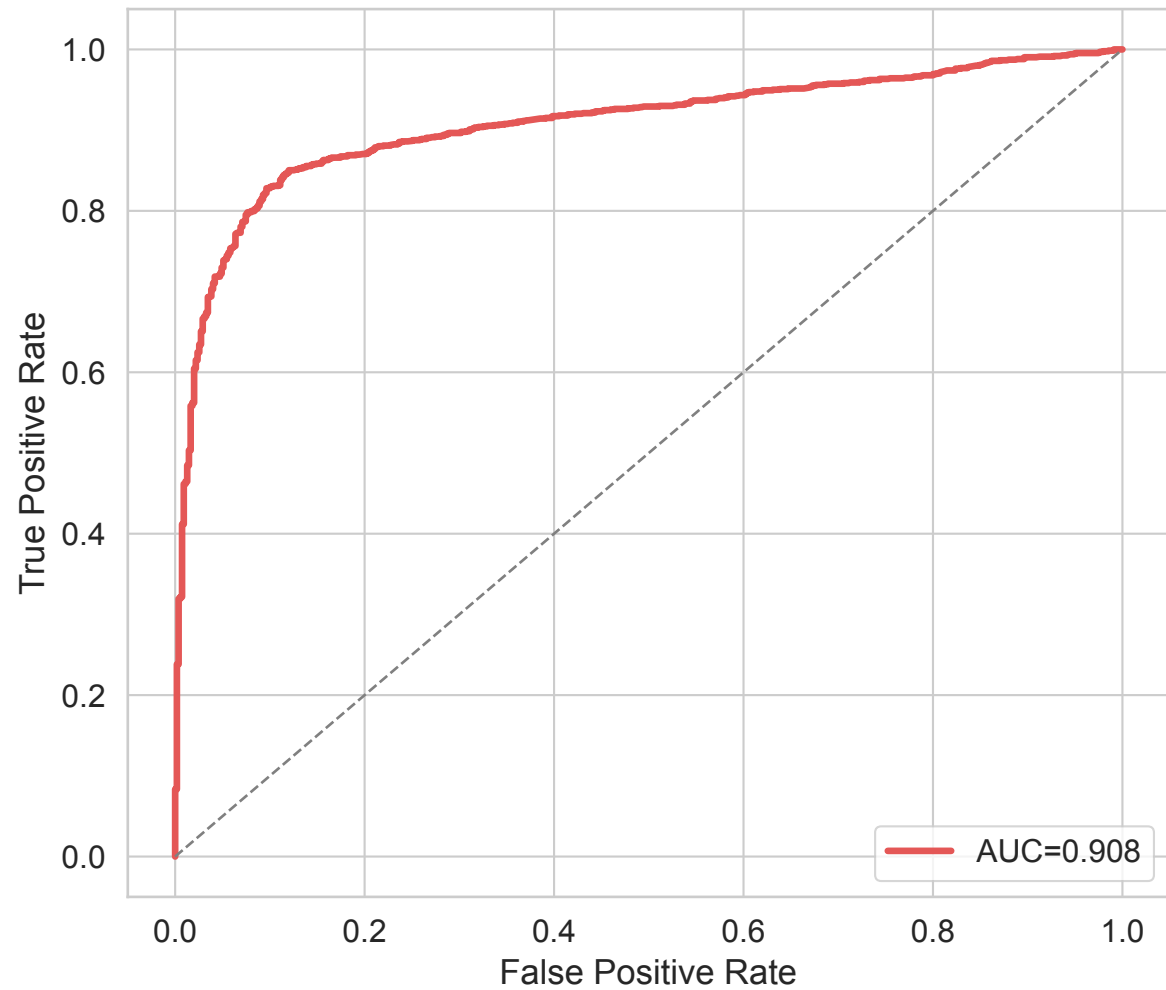
ET: ROC Curve
