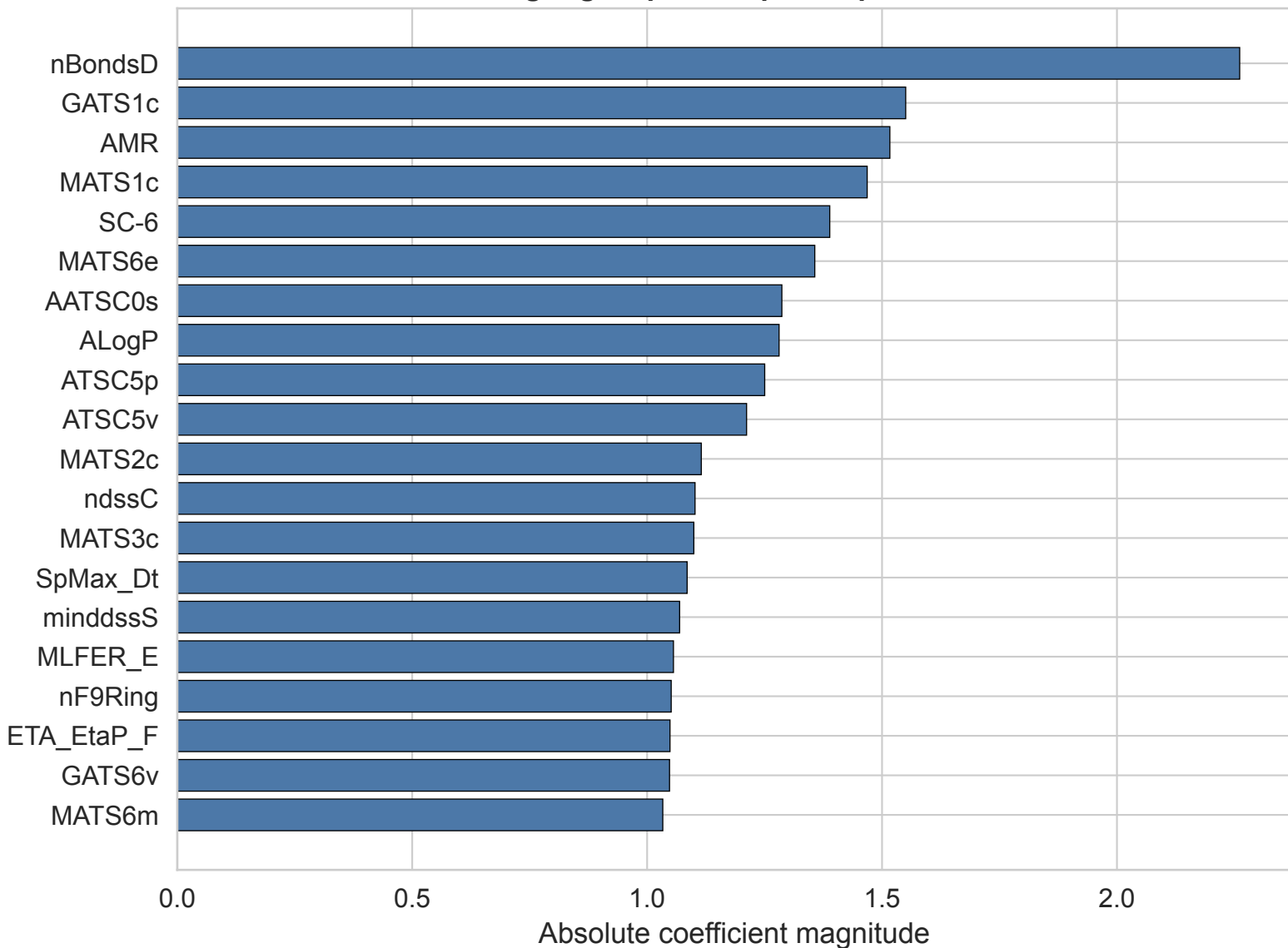
LogReg: Top Descriptor Importance
