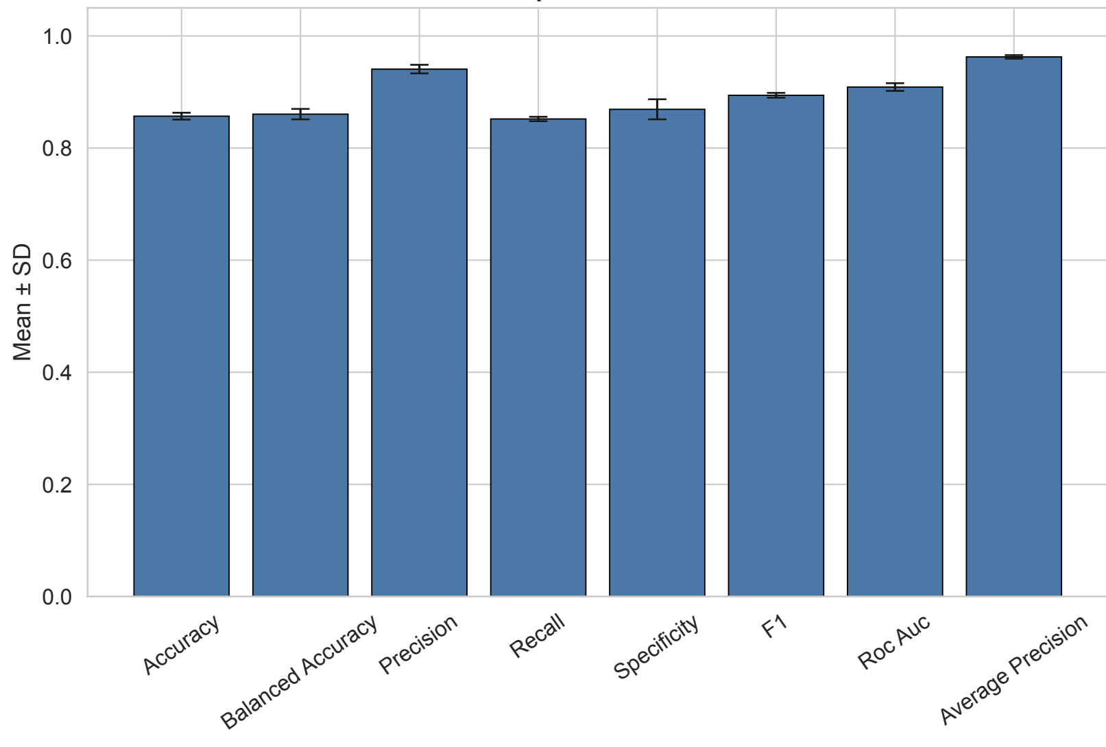
XGB: Bootstrap Trial Mean Metrics \pm SD
