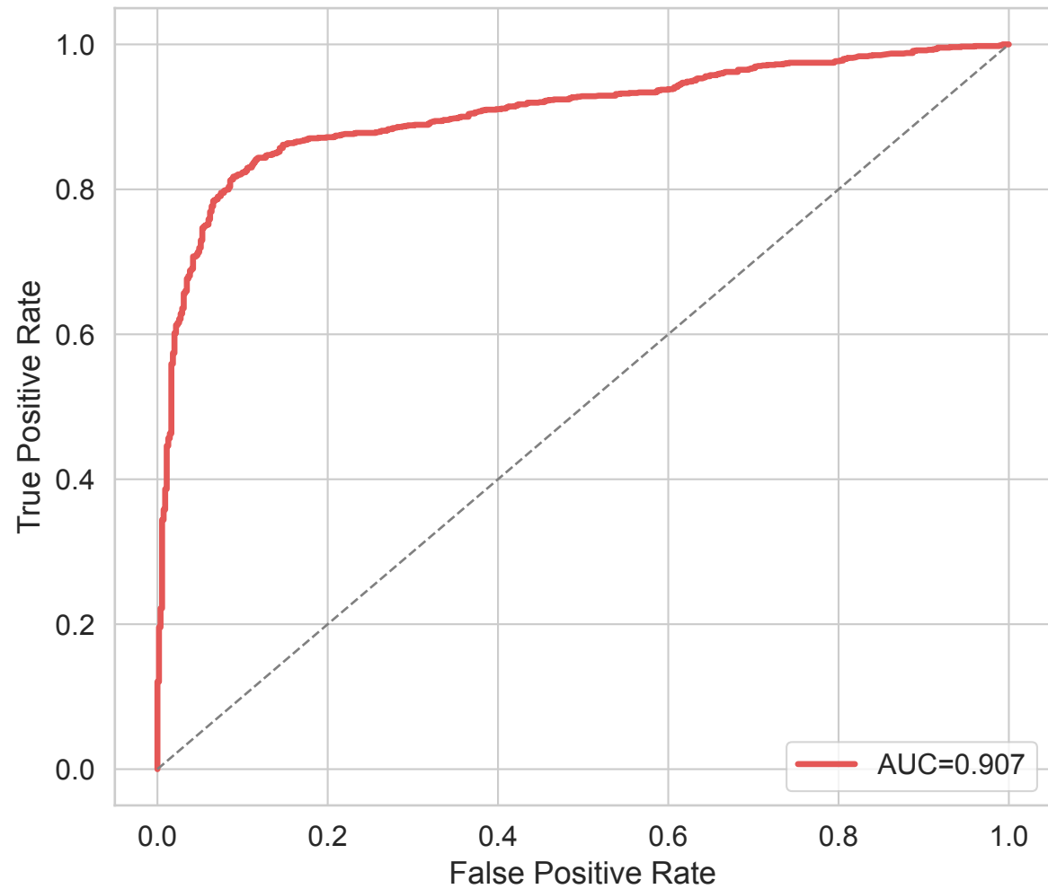
XGB: ROC Curve
