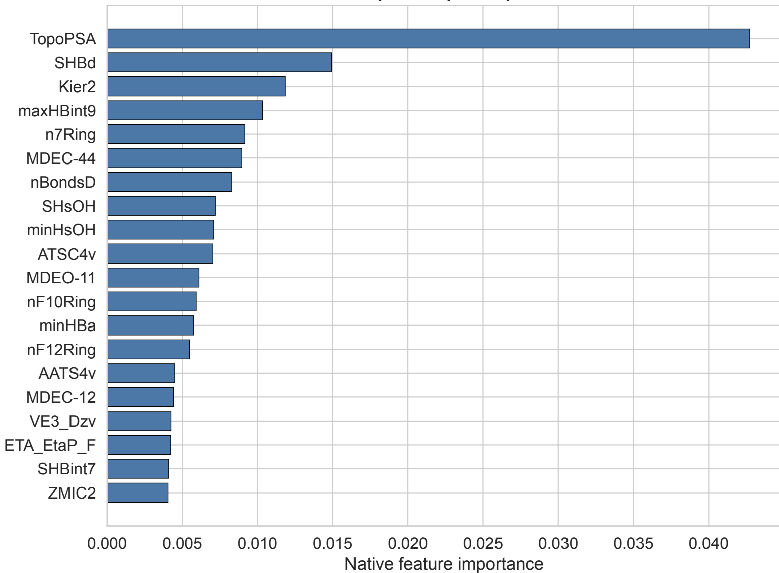
XGB: Top Descriptor Importance
