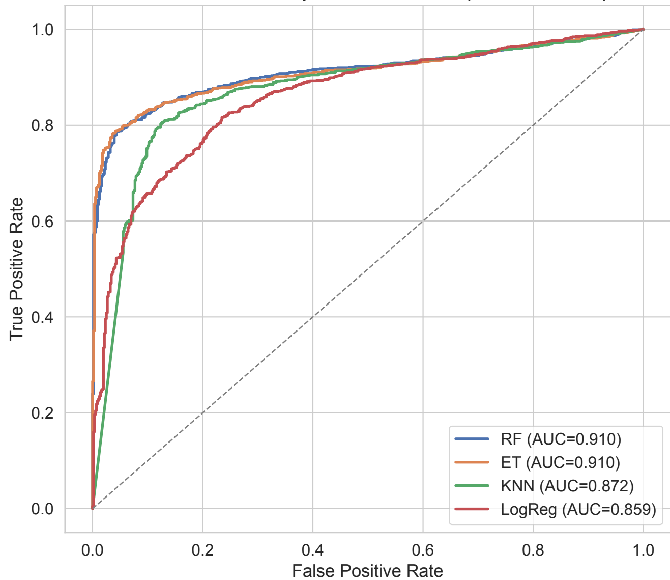
BBB-Relevant Descriptors: ROC Curves (Official Test Set)
