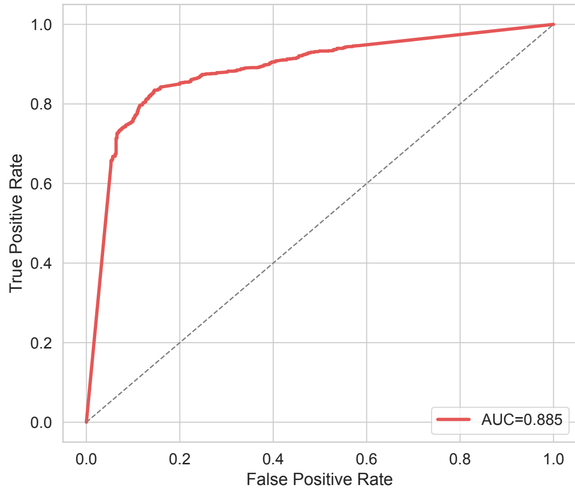
KNN: ROC Curve
