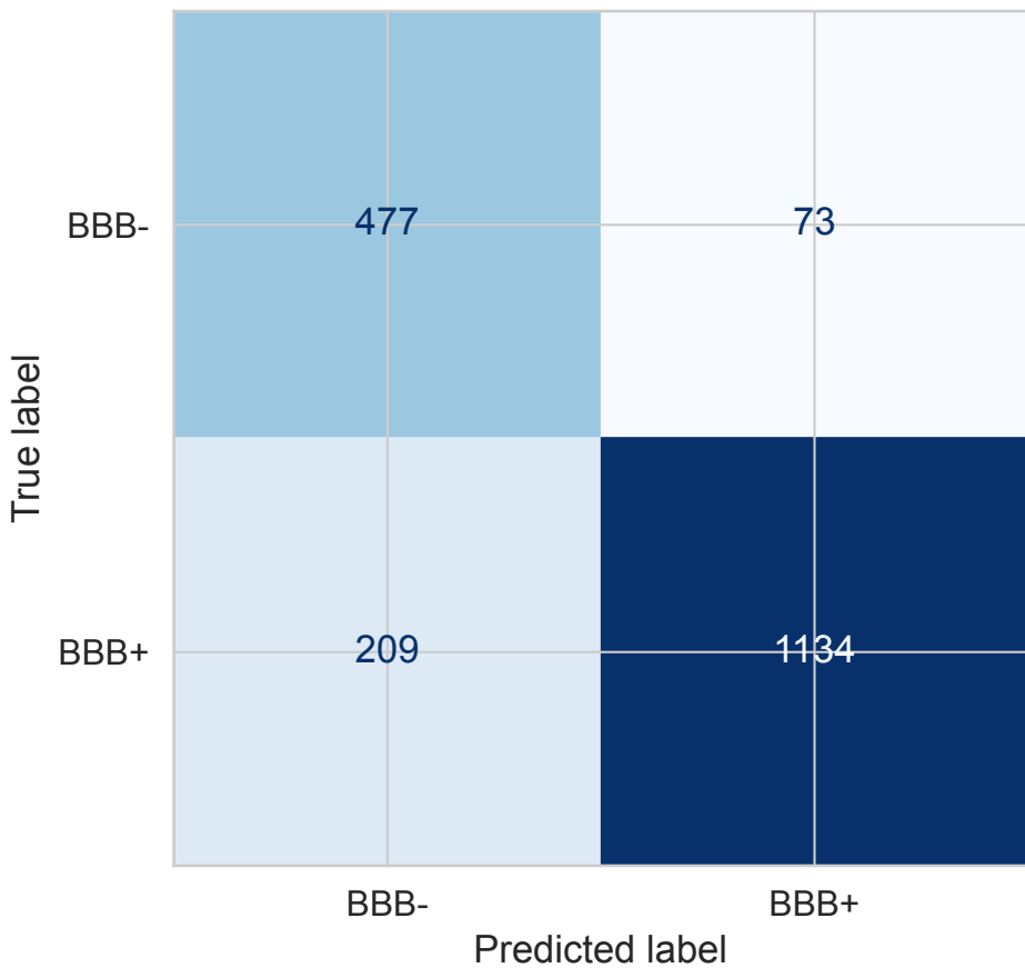
RF: Confusion Matrix
