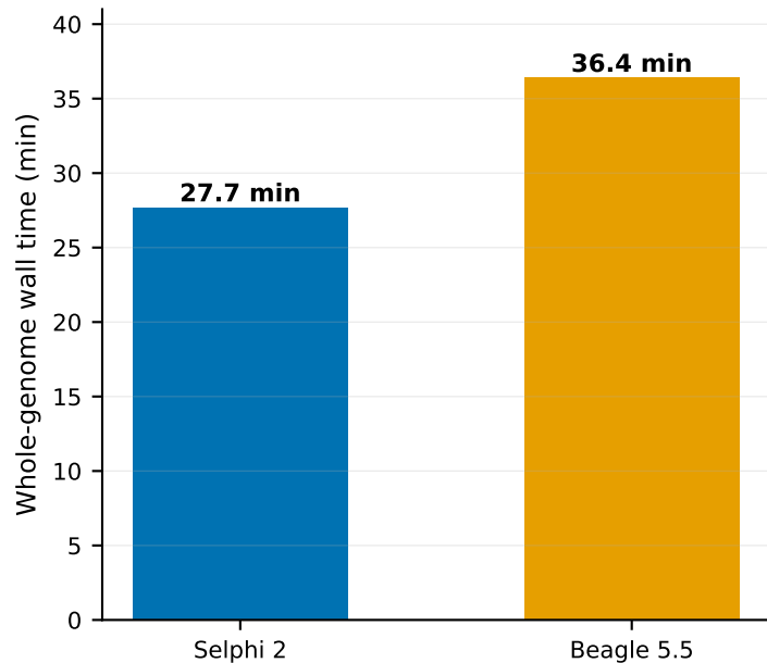
(a) Whole-genome wall time
