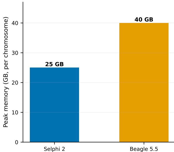
(b) Peak memory
