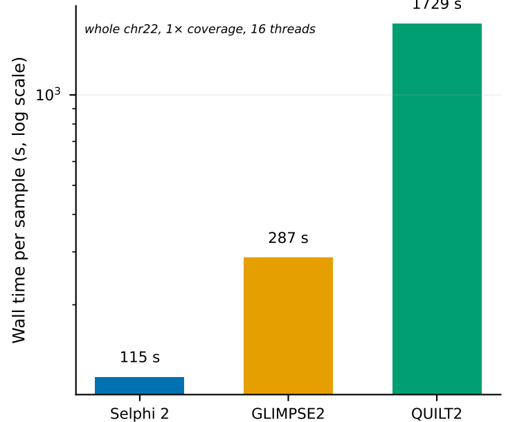
(c) IcWGS speed, whole chr22 (1 sample)
