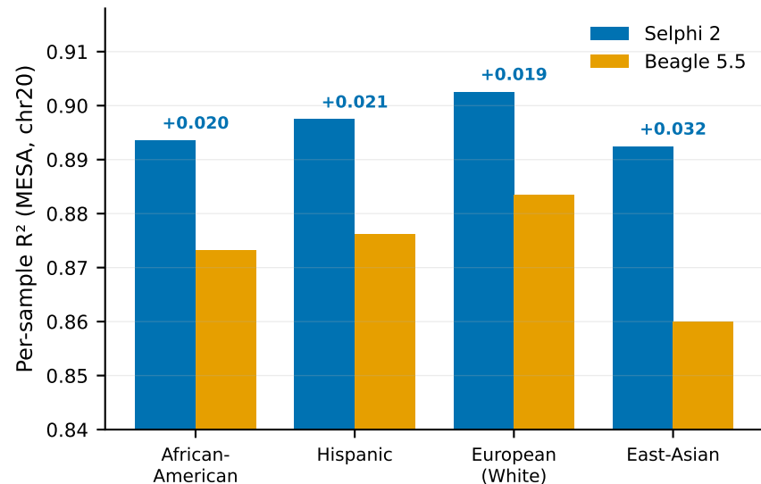
(b) Per-sample accuracy by ancestry, MESA
