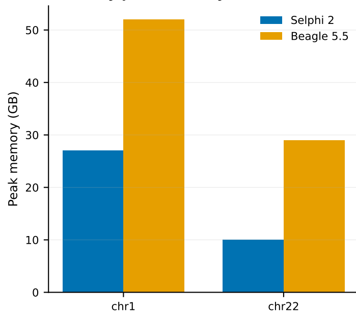
(b) Array peak memory
