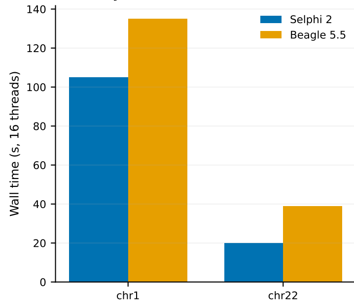
(a) Array wall time
