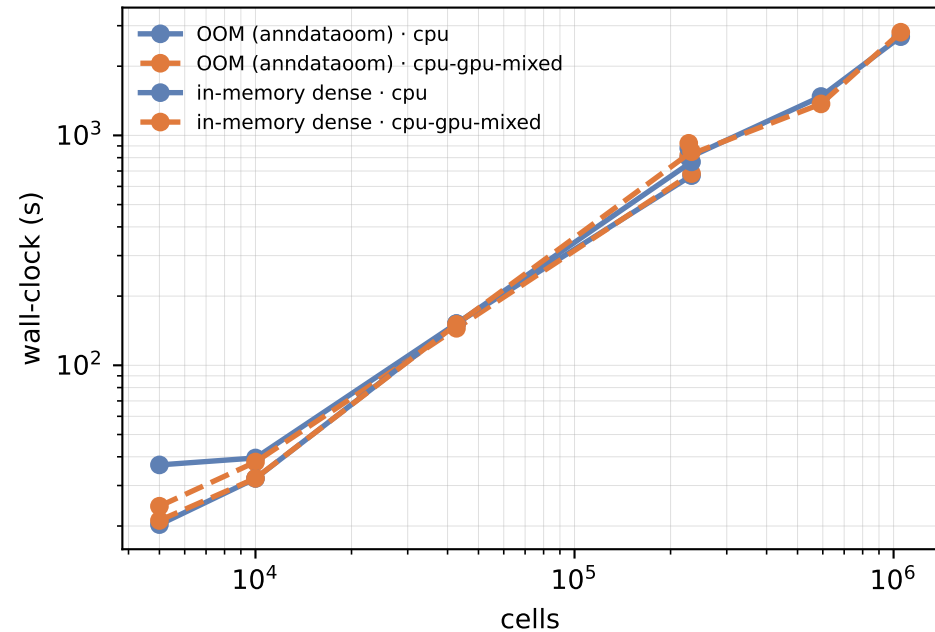
(a) cpu vs cpu-gpu-mixed: pipeline time
