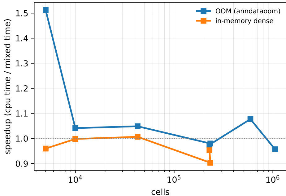
(b) mixed-mode speedup (>1 = mixed faster)
